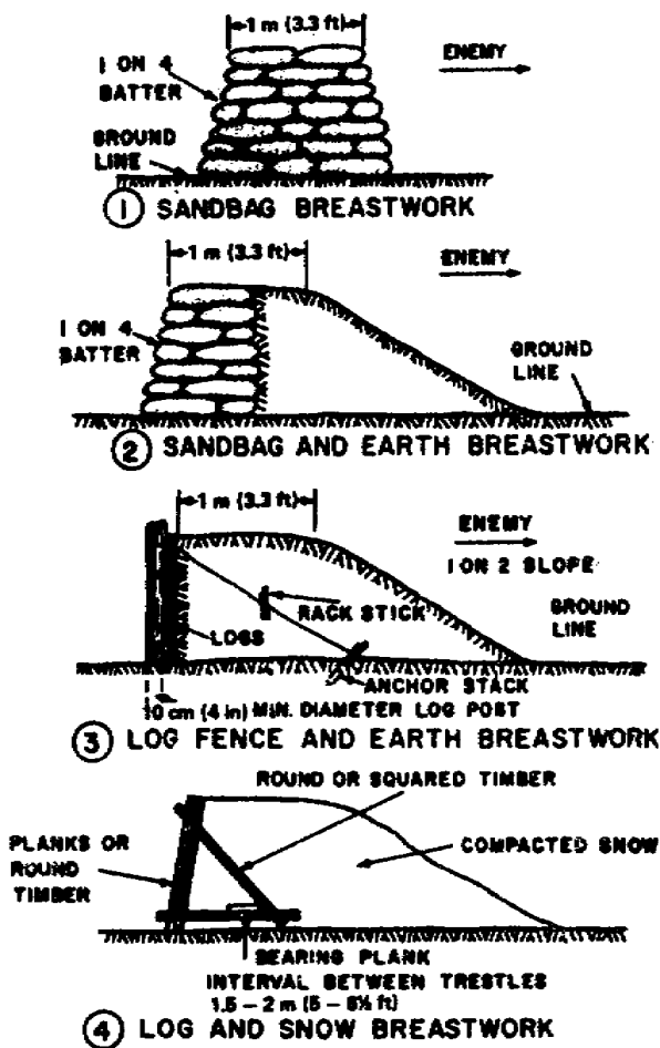
Figure 2-26. Varied types of breastworks.
